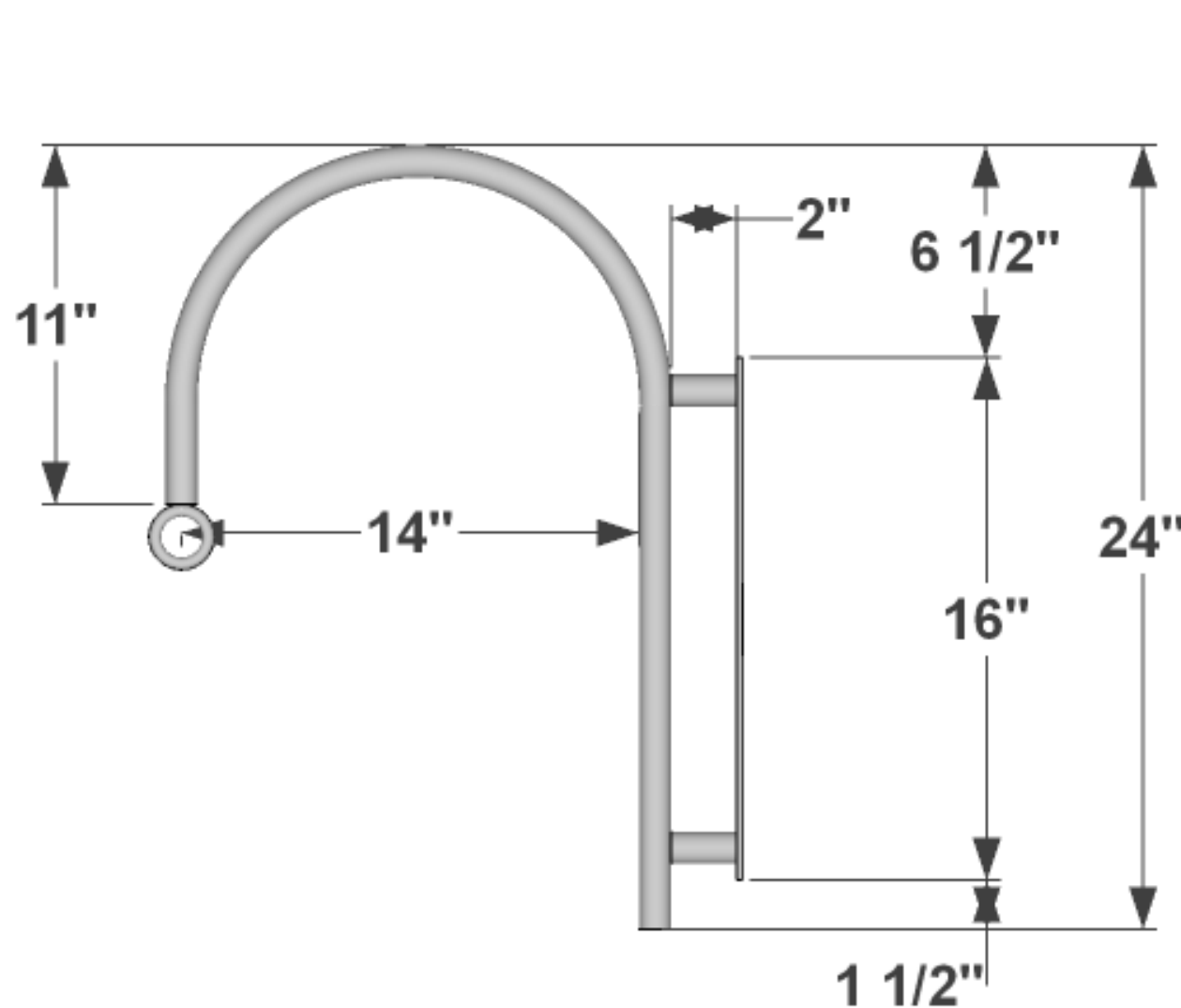
SIDE VIEW
