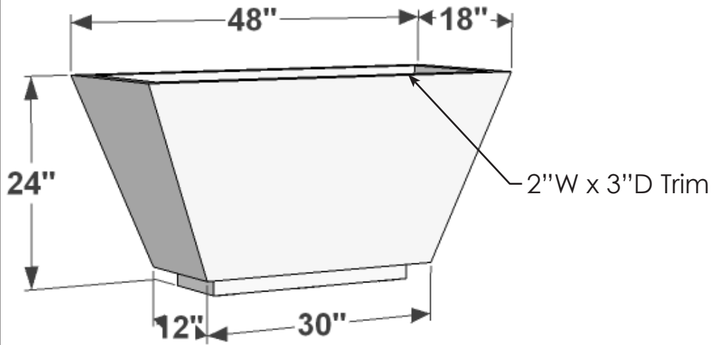
PERSPECTIVE VIEW
