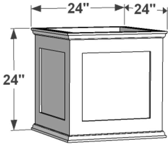
PERSPECTIVE VIEW
