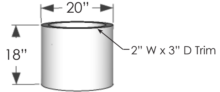
PERSPECTIVE VIEW
