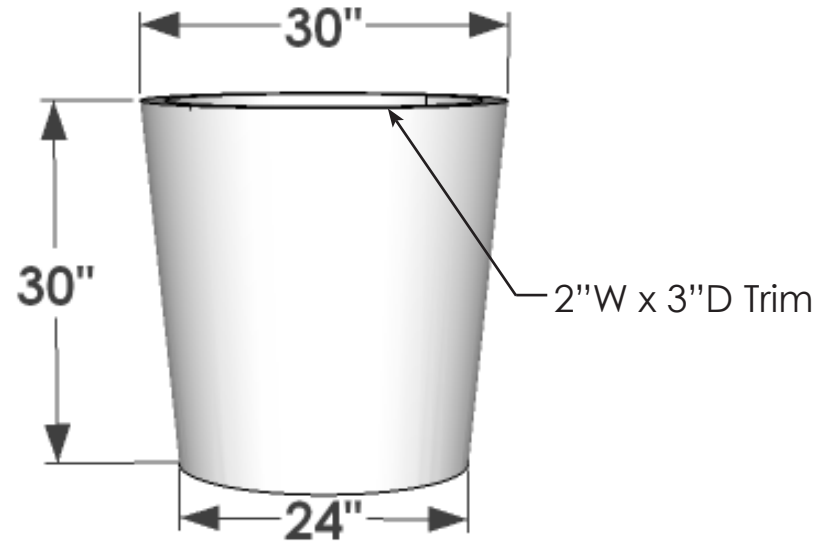
PERSPECTIVE VIEW
