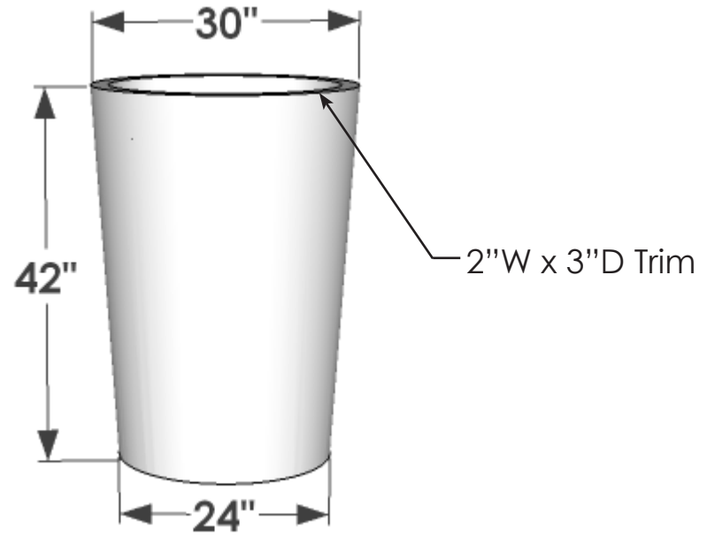
PERSPECTIVE VIEW
