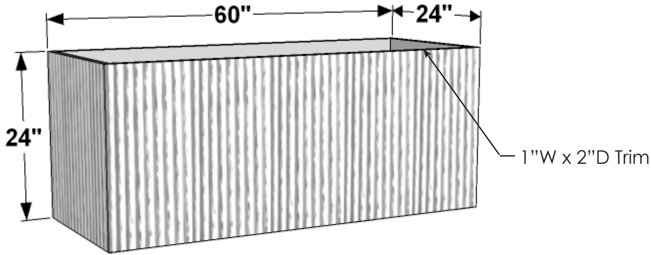
PERSPECTIVE VIEW
