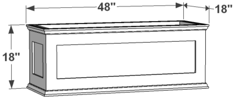
PERSPECTIVE VIEW
