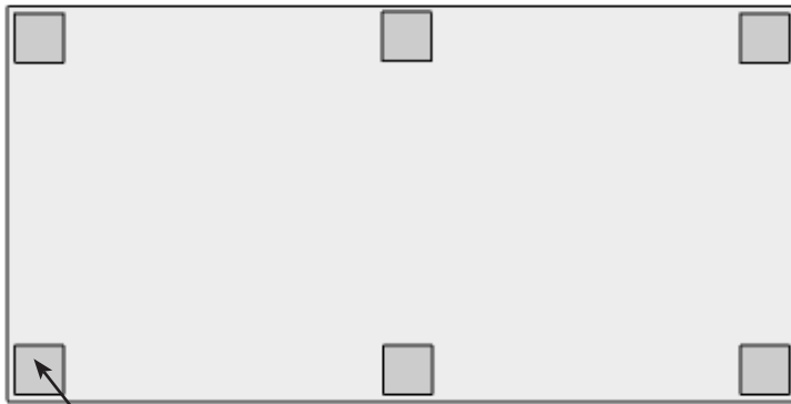
(6) Pads, 4"x4"x1/8"thk. Offset 1" from edges.
