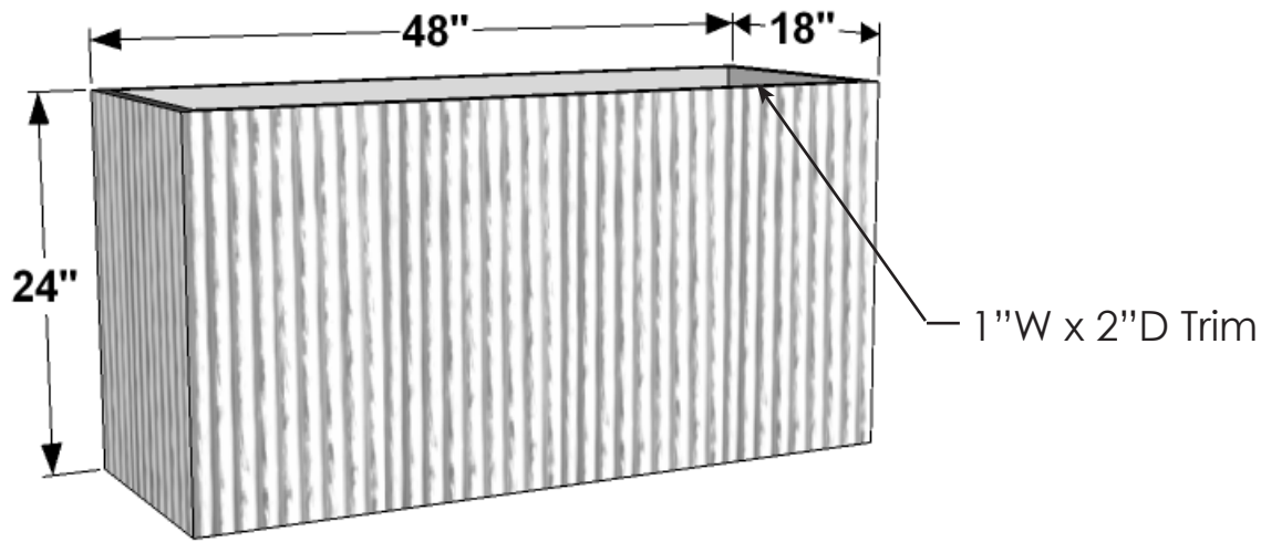
PERSPECTIVE VIEW
