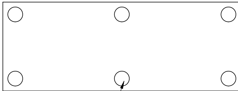
(6) Pads, 3" Dia. x 1/4" thk. Offset 1" from edges
