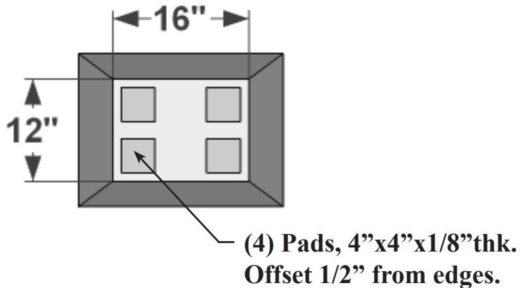
BOTTOM VIEW
