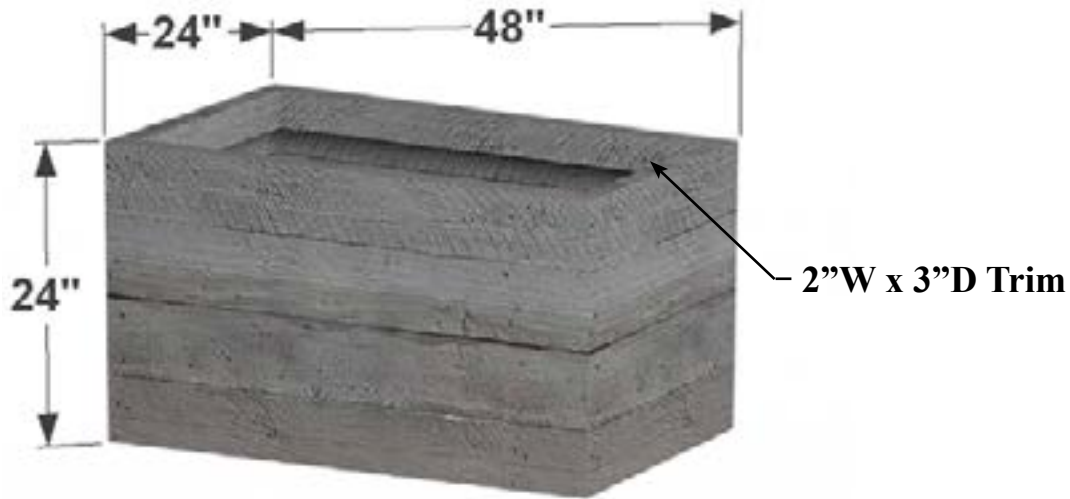
PERSPECTIVE VIEW
