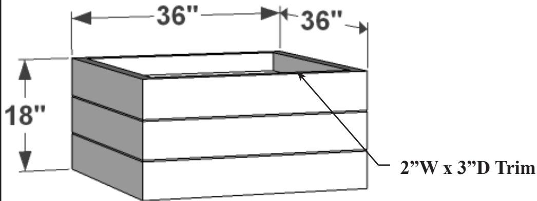
PERSPECTIVE VIEW
