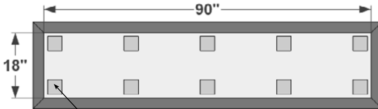
(10) Pads, 4"x4"x1/8" thk. Offset 1" from edges.
