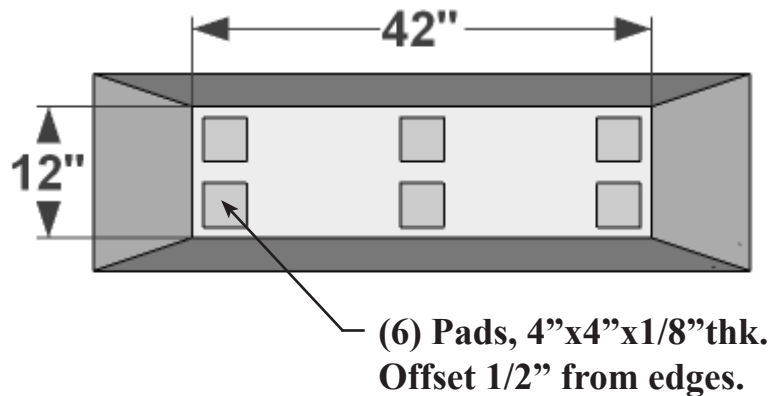
BOTTOM VIEW
