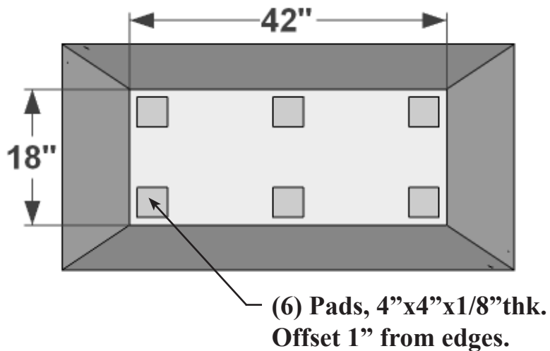
BOTTOM VIEW
