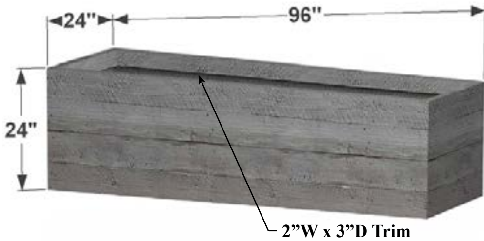
PERSPECTIVE VIEW
