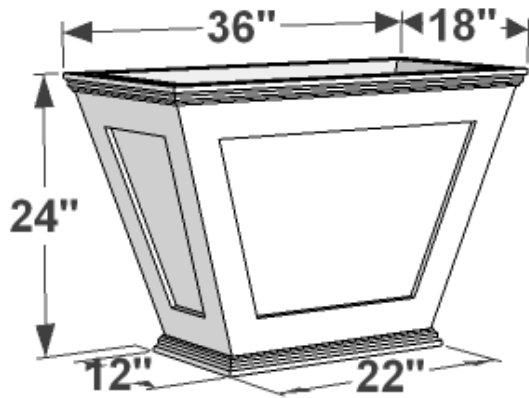
PERSPECTIVE VIEW
