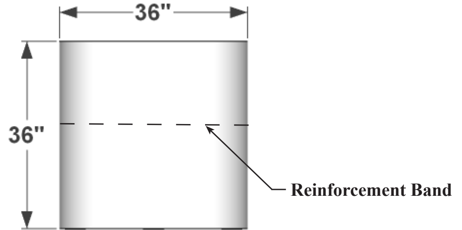
ELEVATION VIEW
