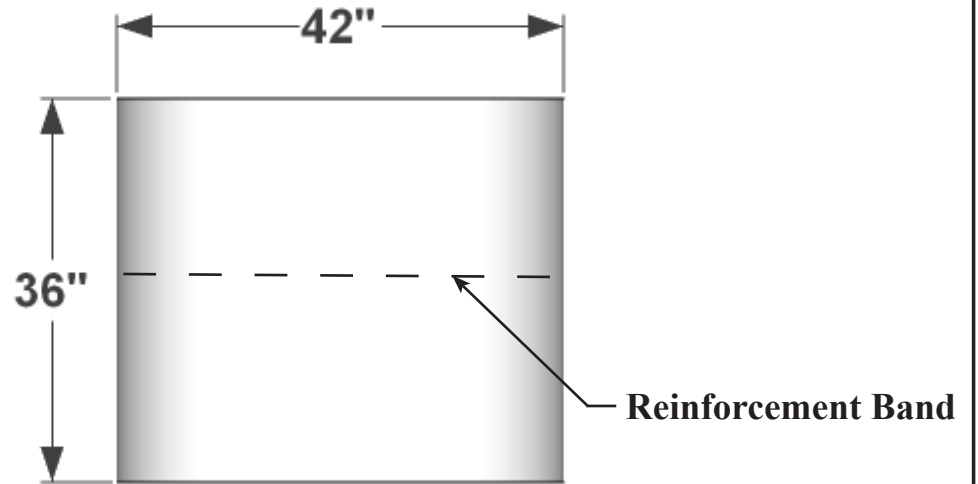
ELEVATION VIEW
