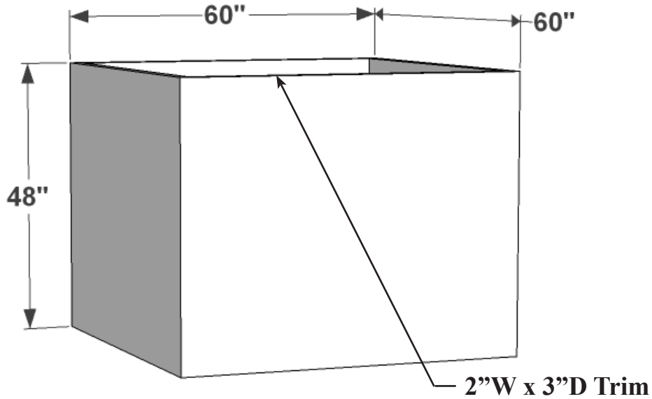
PERSPECTIVE VIEW
