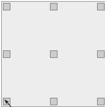
(9) Pads, 4"x4"x1/8"thk. Offset 1" from edges.
