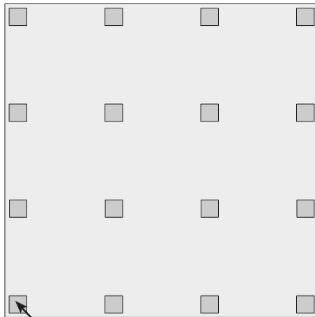
(16) Pads, 4"x4"x1/8"thk. Offset 1" from edges.
