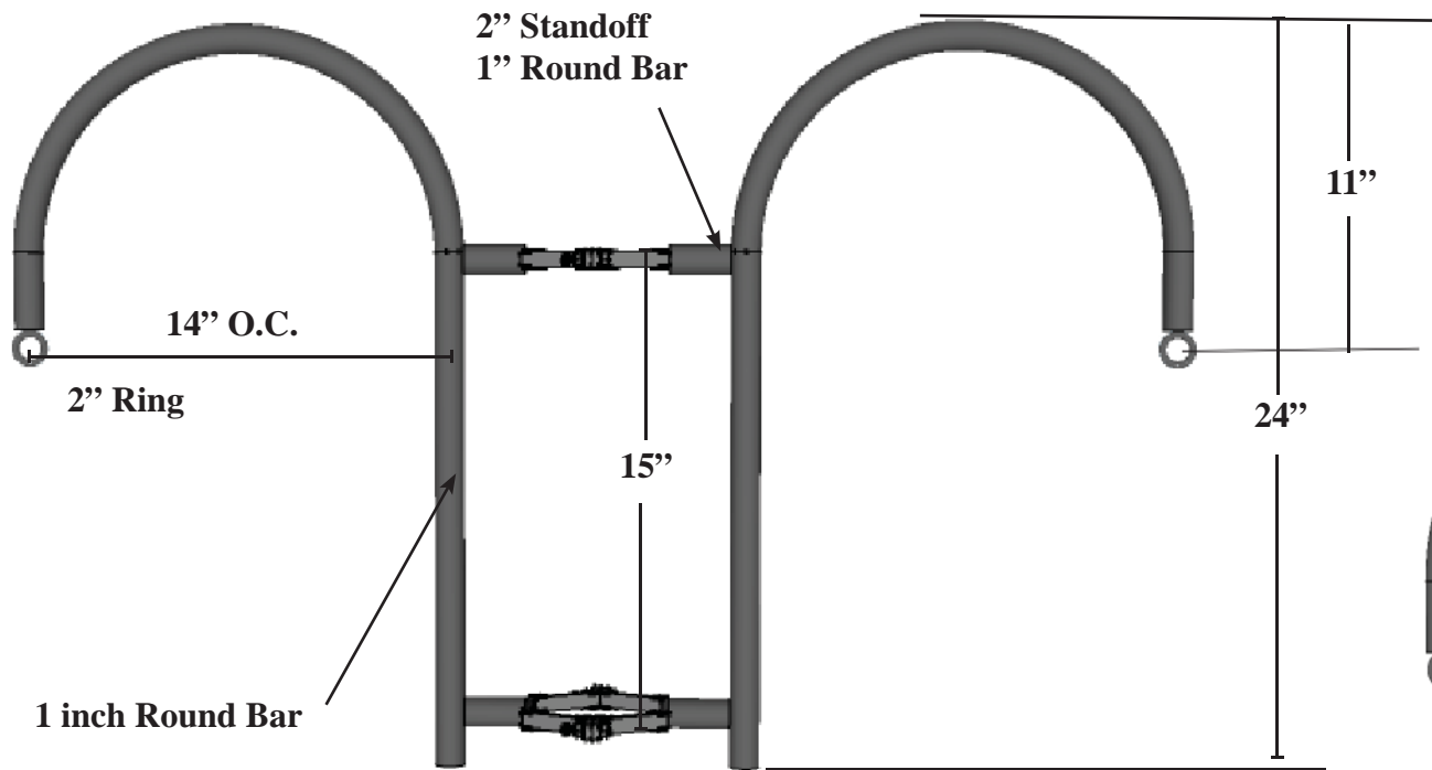
BRACKET PROFILE
