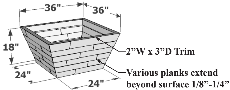
FRONT PERSPECTIVE
