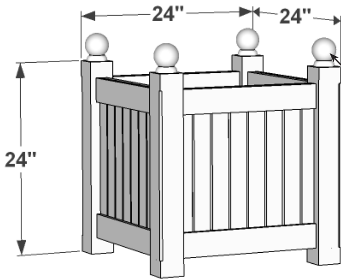
PERSPECTIVE VIEW
