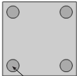
(4) Pads, 3" dia. x 1/4" thk. Offset 1" from edges
