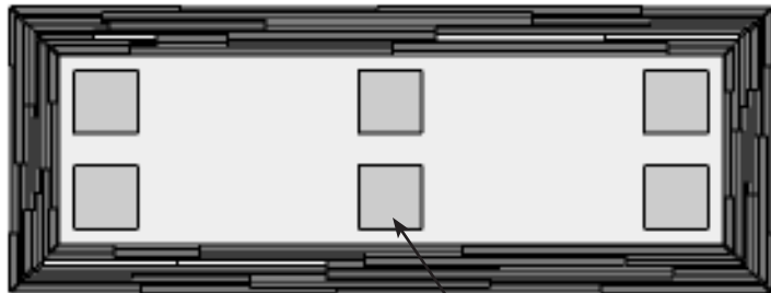
(6) Pads, 4"x4"x1/8"thk. Offset 1" from edges.
