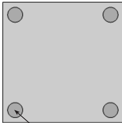
(4) Pads, 3" dia. x 1/4" thk. Offset 1" from edges
