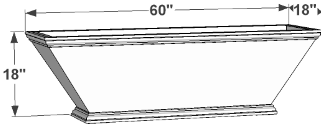
PERSPECTIVE VIEW
