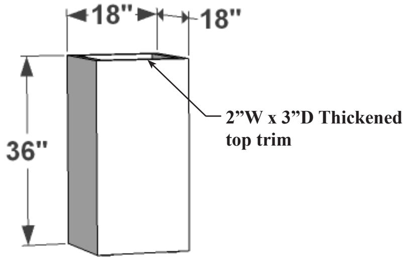
PERSPECTIVE VIEW
