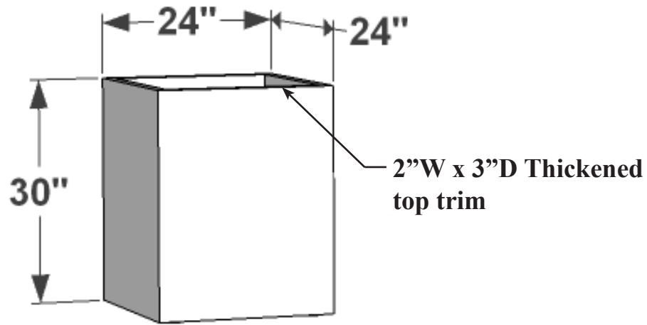
PERSPECTIVE VIEW
