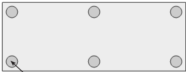
(6) Pads, 3"dia. x 1/4"thk. Offset 1" from edges
