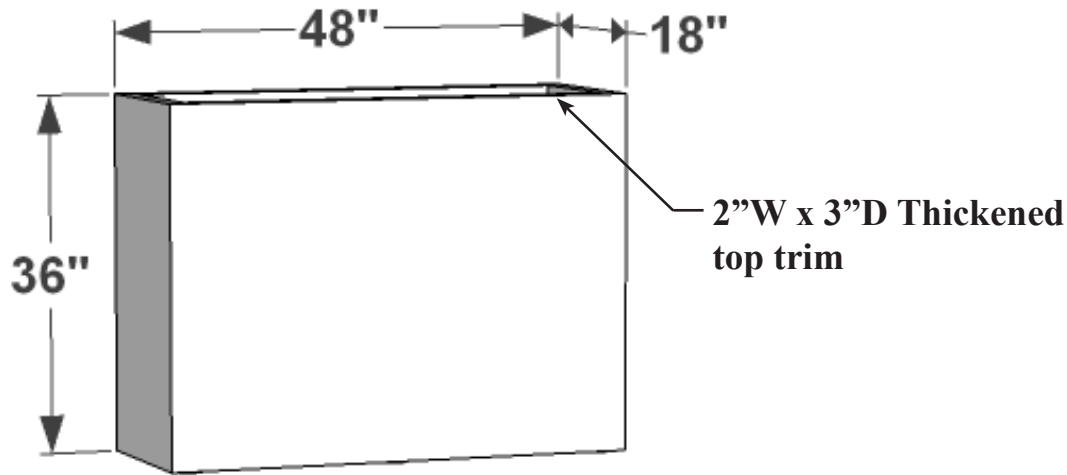
PERSPECTIVE VIEW
