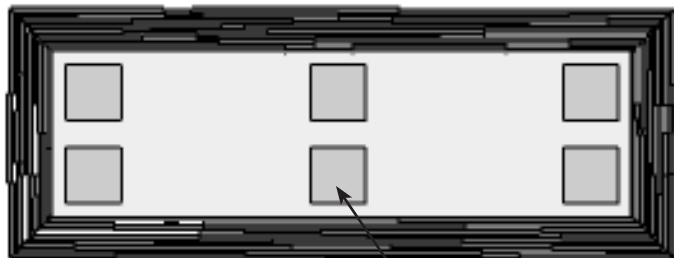
(6) Pads, 4"x4"x1/8"thk. Offset 1" from edges.
