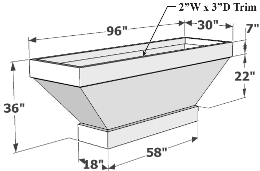
PERSECTIVE VIEW
