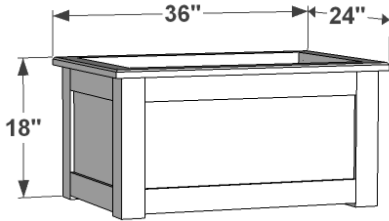
PERSPECTIVE VIEW
