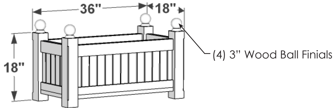
PERSPECTIVE VIEW
