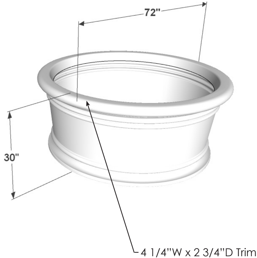
PERSPECTIVE VIEW
