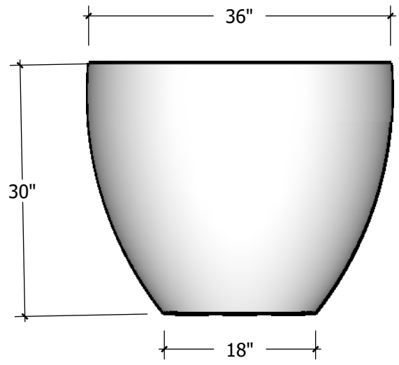
ELEVATION VIEW
