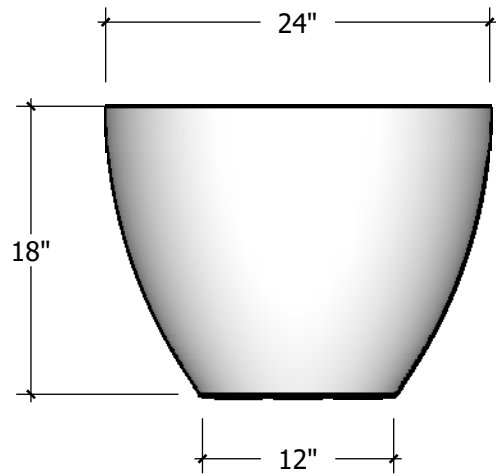
ELEVATION VIEW
