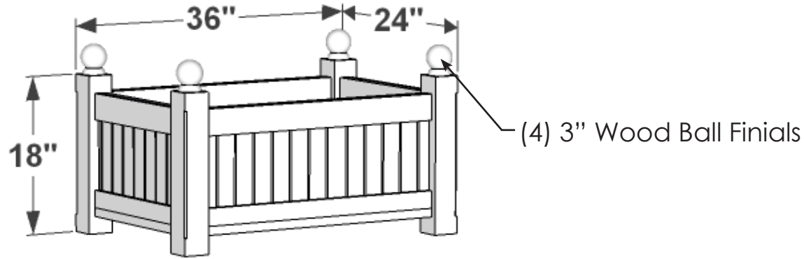
PERSPECTIVE VIEW
