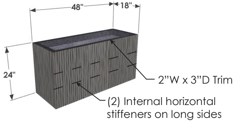
PERSPECTIVE VIEW
