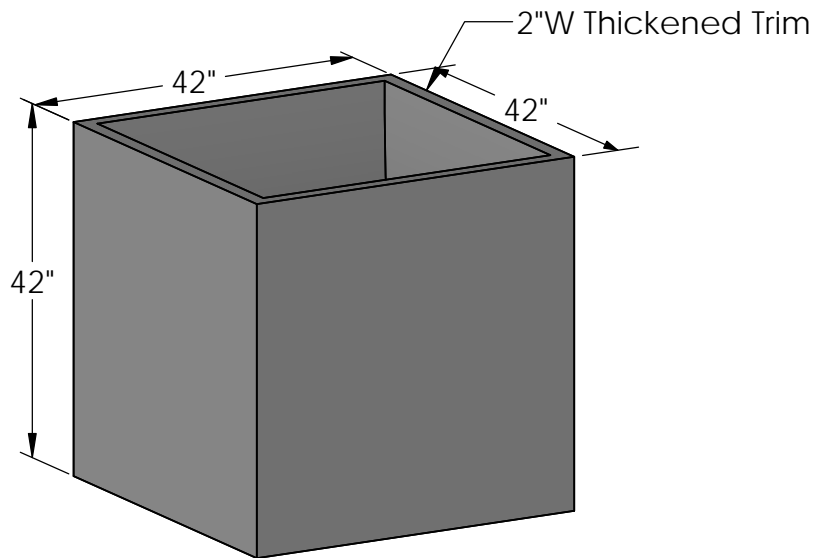
PERSPECTIVE VIEW
