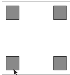
(4) Pads, 3"x3"x1/8"thk. Offset 1" from edges.
