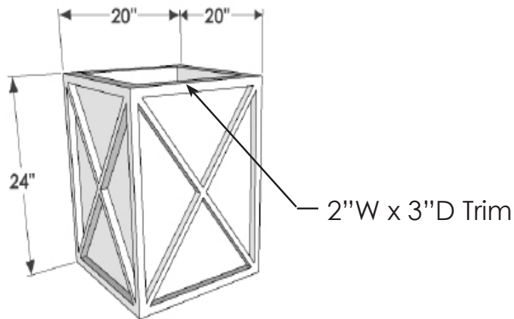
PERSPECTIVE VIEW
