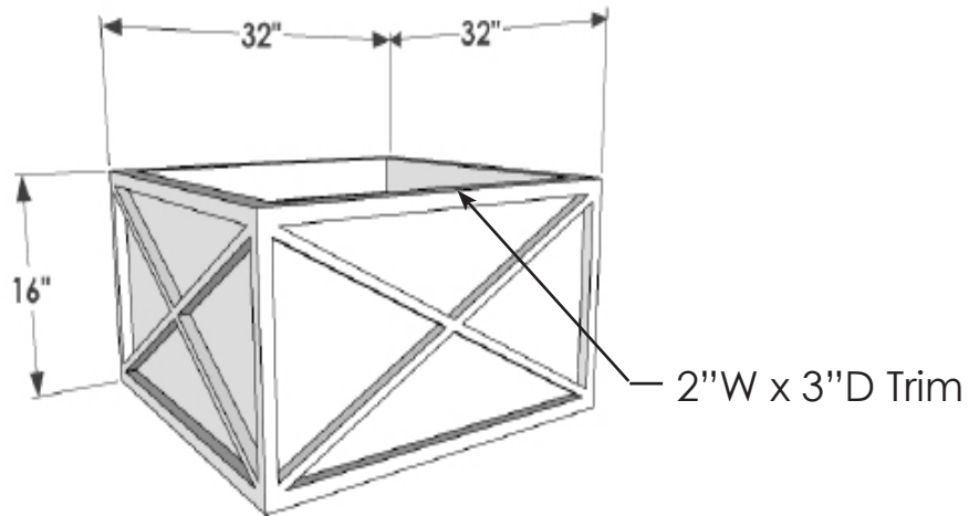
PERSPECTIVE VIEW
