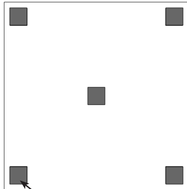
(5) Pads, 3"x3"x1/8"thk. Offset 1" from edges.
