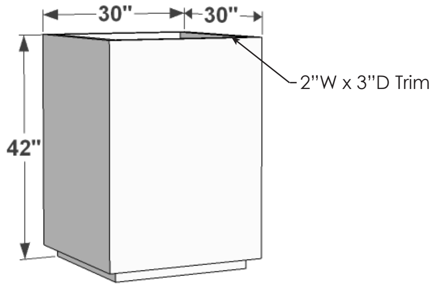
PERSPECTIVE VIEW
