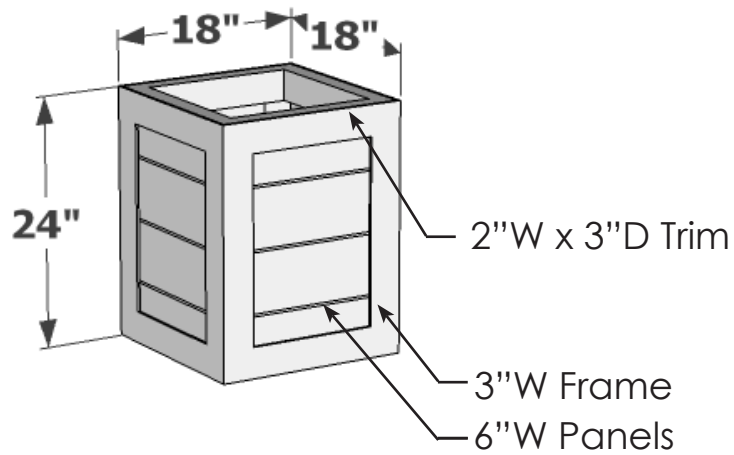
PERSPECTIVE VIEW
