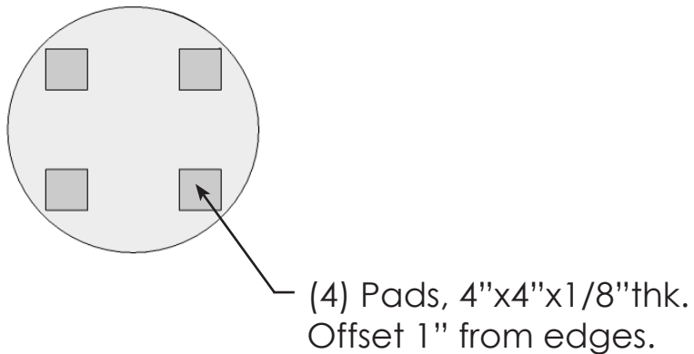
BOTTOM VIEW
