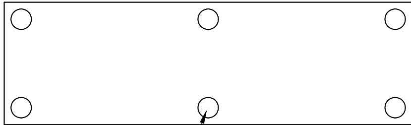
(6) Pads, 3"Dia. x 1/4"thk. Offset 1" from edges
